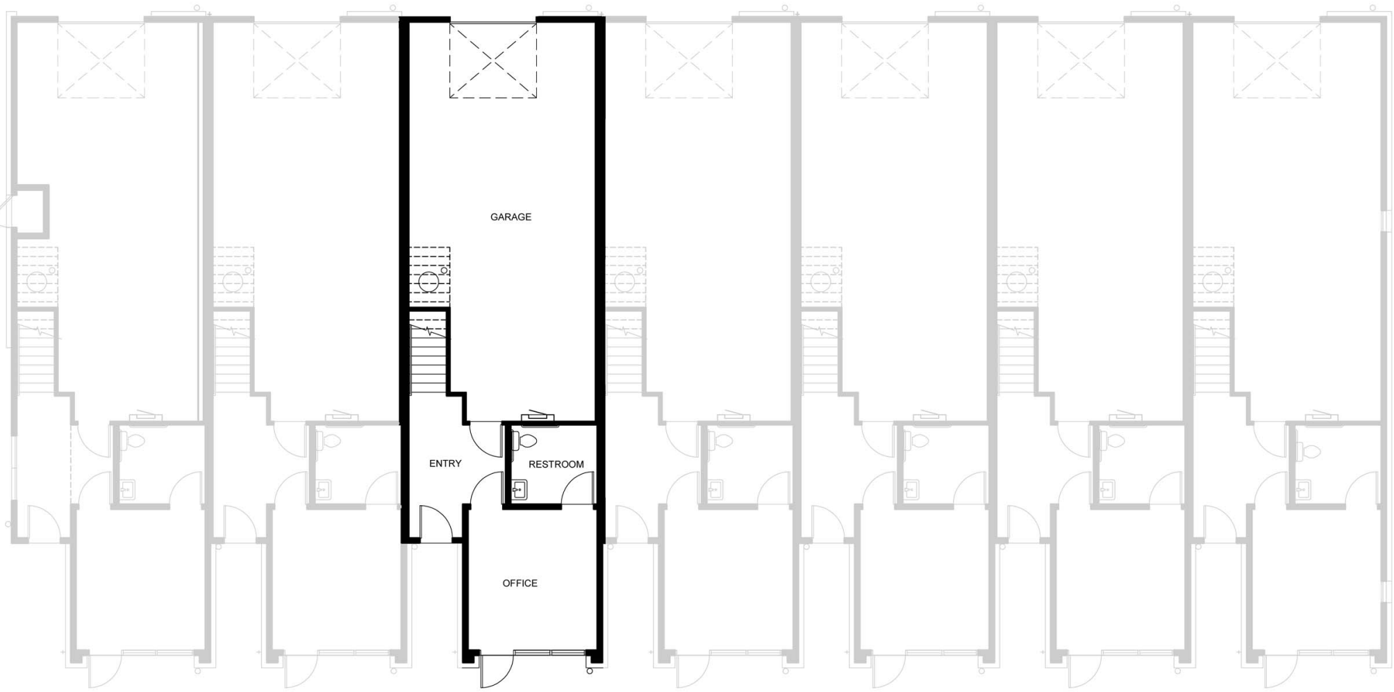
TOWN LAKE L/W UNIT 1ST FLOOR PLAN
