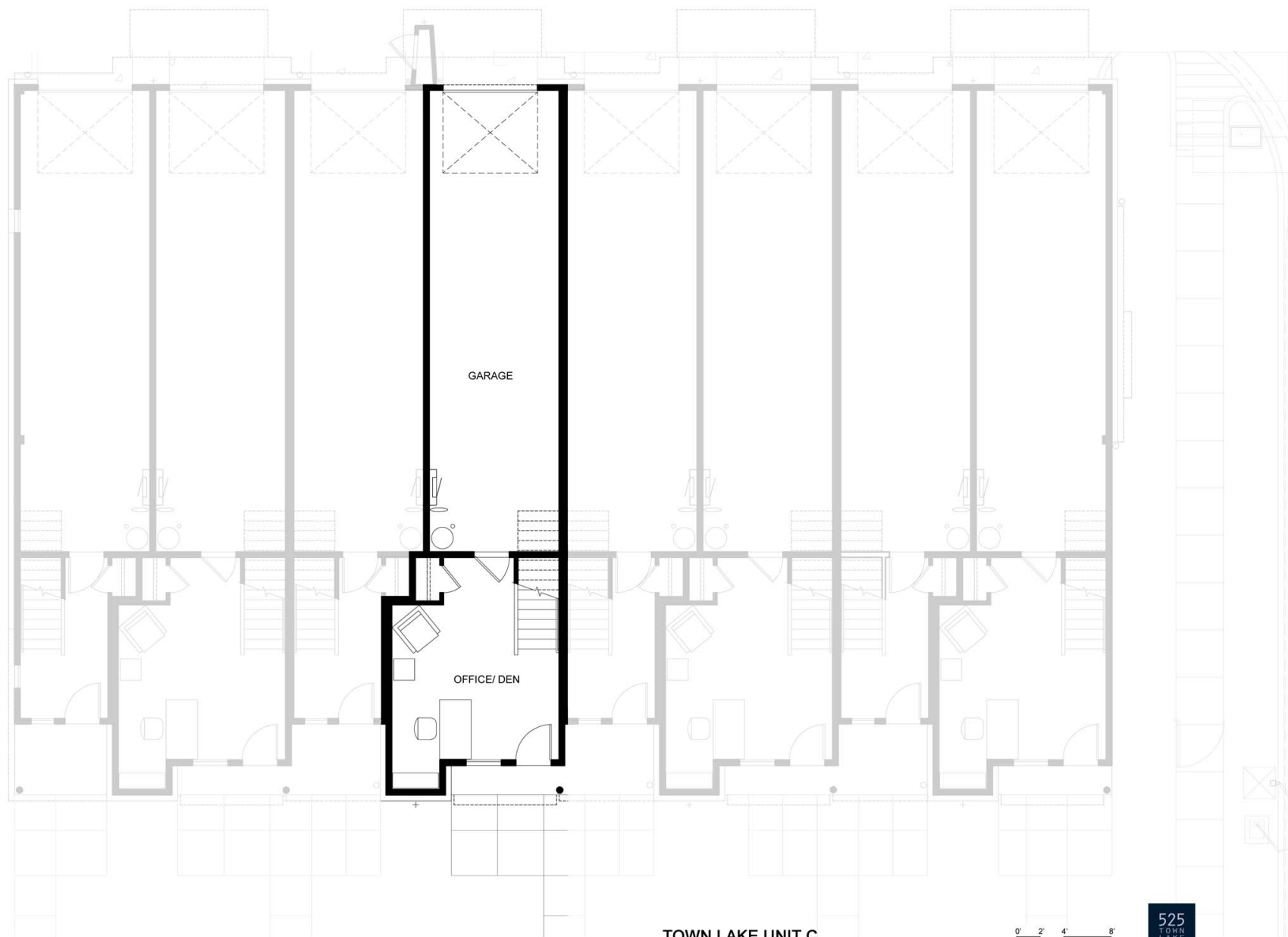
TOWN LAKE UNIT C 1ST FLOOR PLAN
