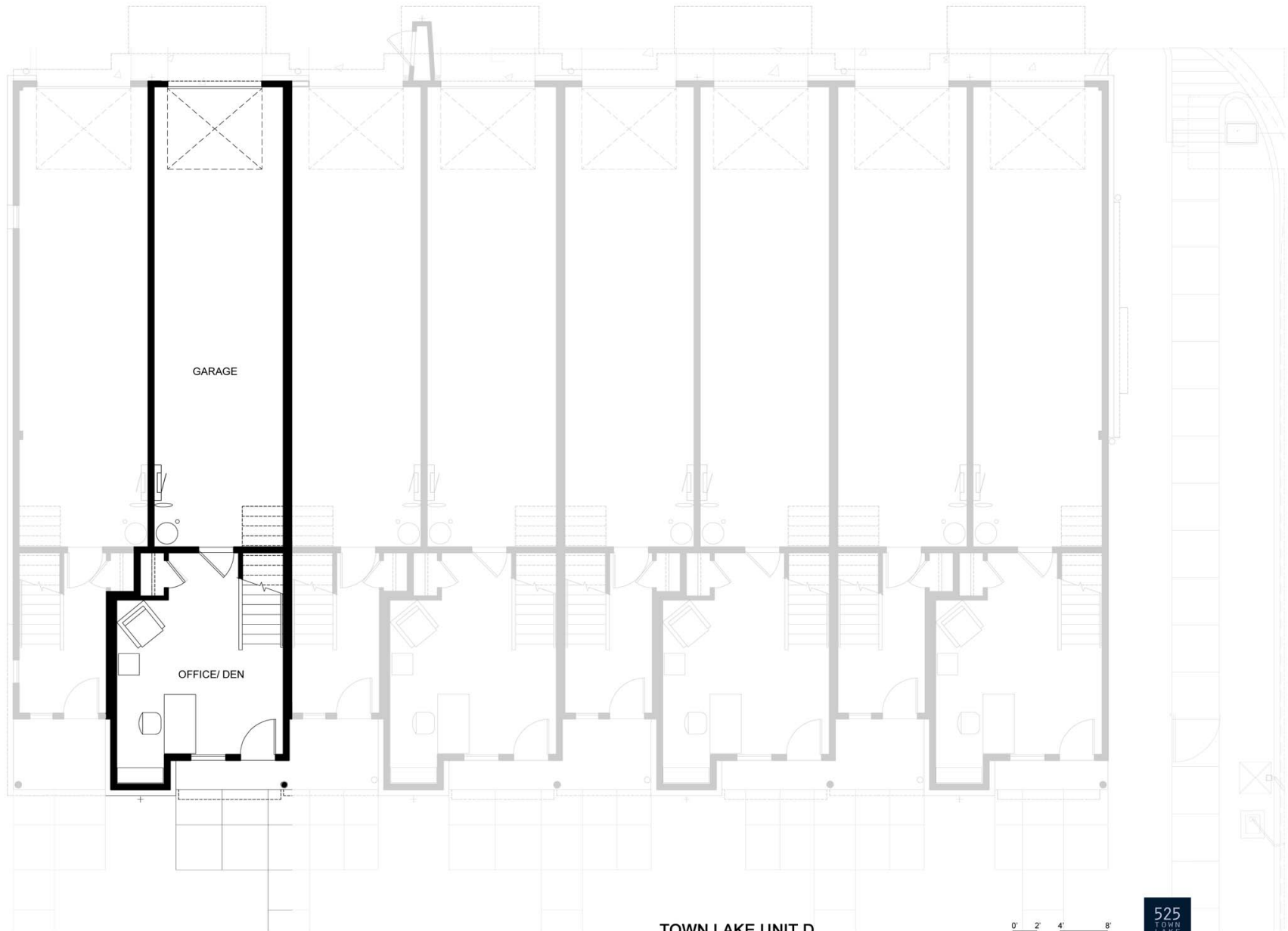
TOWN LAKE UNIT D 1ST FLOOR PLAN
